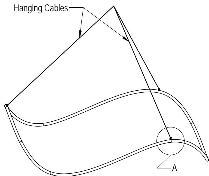
Isometric View Scale 1 : 32
