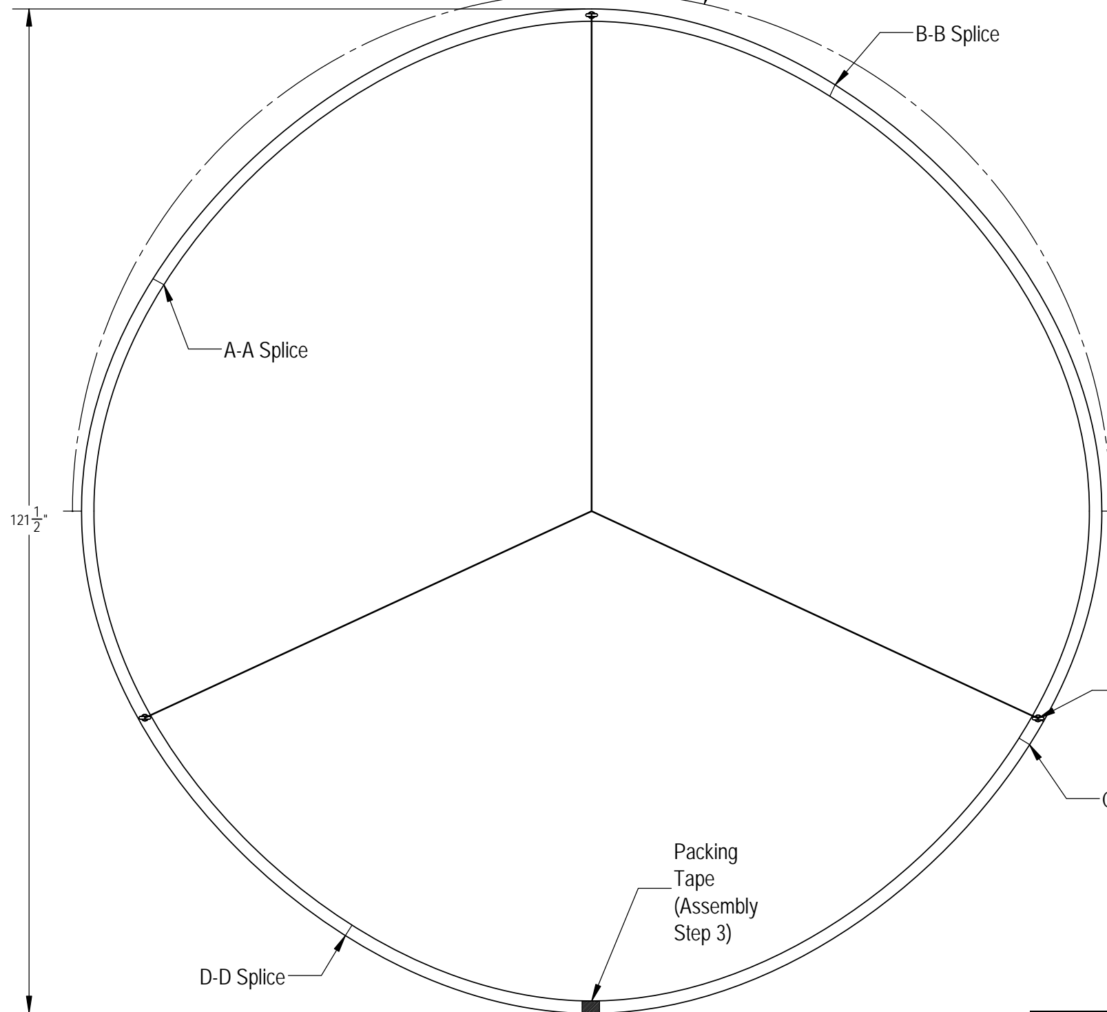
Top View Scale 1 : 16
