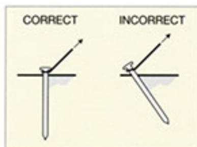
Figure 13. Stake Driving Angle
