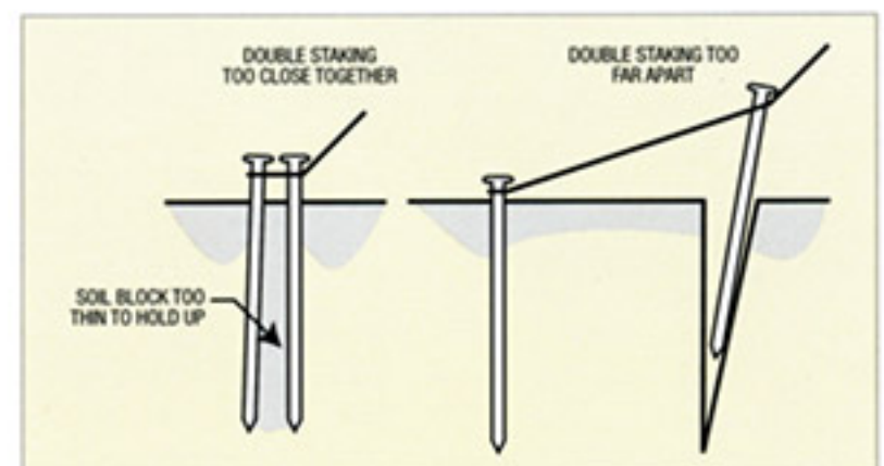
Figure 18. Double Staking Errors
